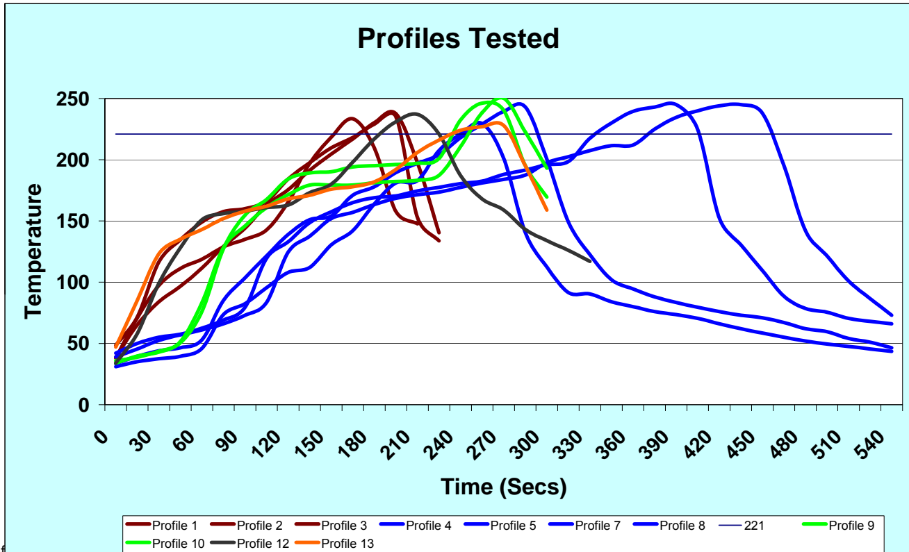
Figure #1 – Reflow Envelope
